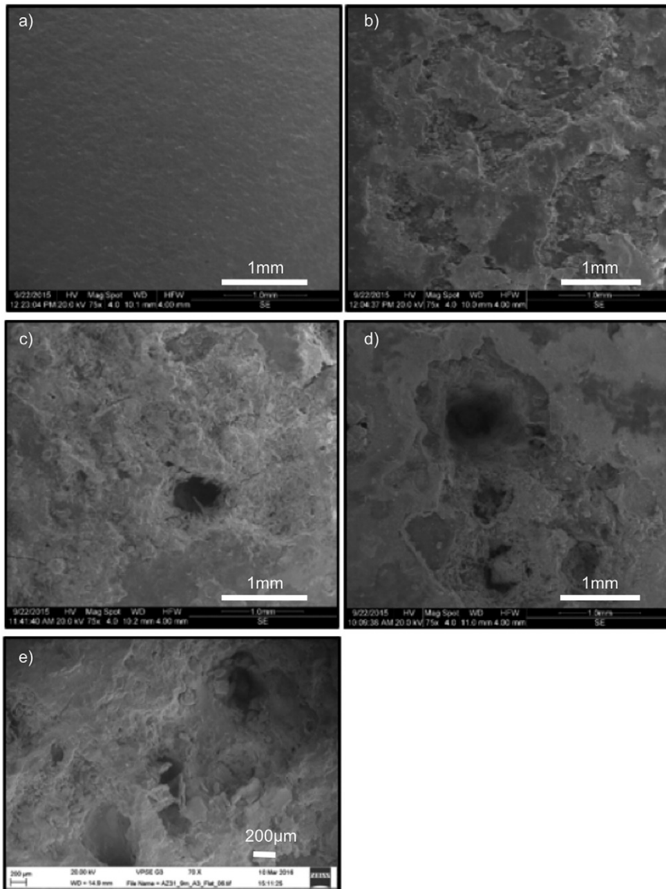
Fig. 6. SEM images showing surface morphology in AZ31 dumbbell samples and the development of corrosion pits on the sample surface in a) non-degraded and degraded specimens after b) 1 month, c) 3 months, d) 6 months and e) 9 months of immersion in PBS (scale bars indicated on image as 1 mm or 200 \mu\text{m} ).
