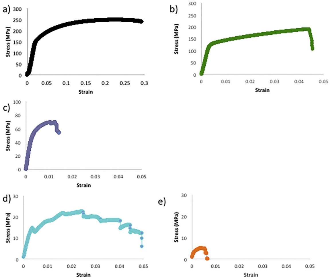
Fig. 4. Typical tensile stress-strain behaviour for AZ31 magnesium alloy after a) 0, b) 1, c) 3, d) 6 and e) 9 months of in vitro degradation in PBS. Data from a median sample in each group.
