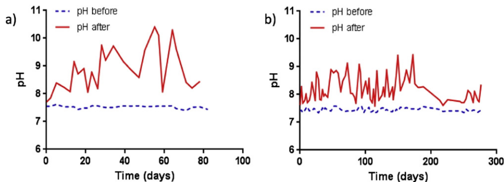
Fig. 2. Degradation media pH for AZ31 Magnesium alloy a) rectangular specimens and b) dumbbell specimens as a function of immersion time before (dashed blue line) and after (solid red line) 2–5 day immersion periods.
